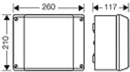
Dimension drawing
