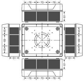
box walls
