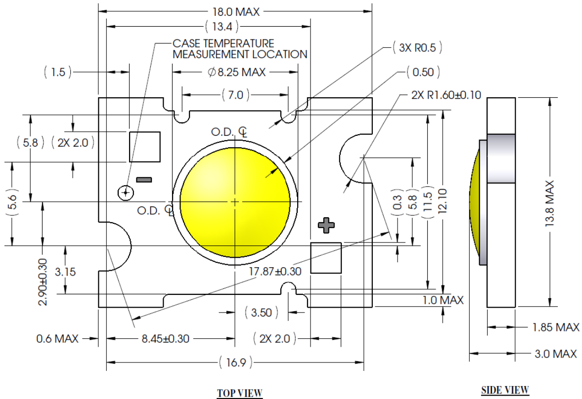
Figure 1: Drawing for part numbers BXRA-W0240, BXRA-W0241, BXRA-W0260, BXRA-W0261, BXRA-C0360 and BXRA-C0361.
