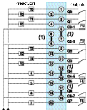
UV: - ~ 19...240 V or ~ 19...60 V for TSX DSY 08R5A - ~ 24...130 V for TSX DSY 08R4D FU: 6.3 A fast-blow fuse (1) Connection must be made for ~ 24 V or ~ 24 V power supply
