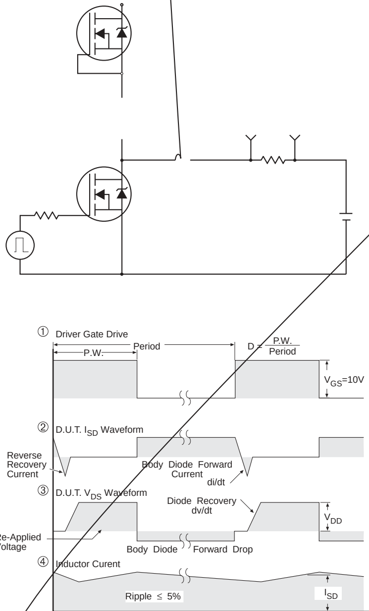
Fig 12. For N-Channel HEXFETS
