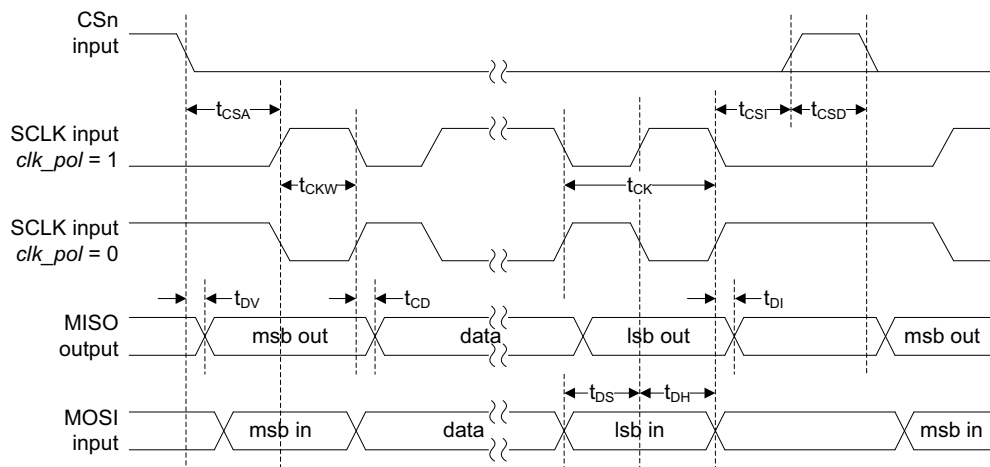
Figure 22: SPI timing diagram, slave mode, clk\_pha = 0
