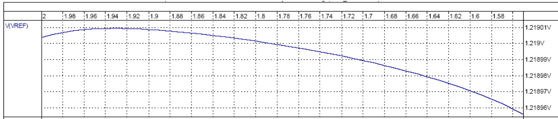
Figure 35: Vref variation with supply voltage (typical)
