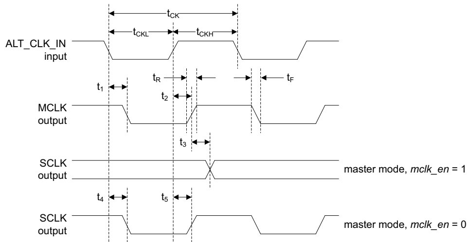
Figure 30: I2S clock signals timing diagram
