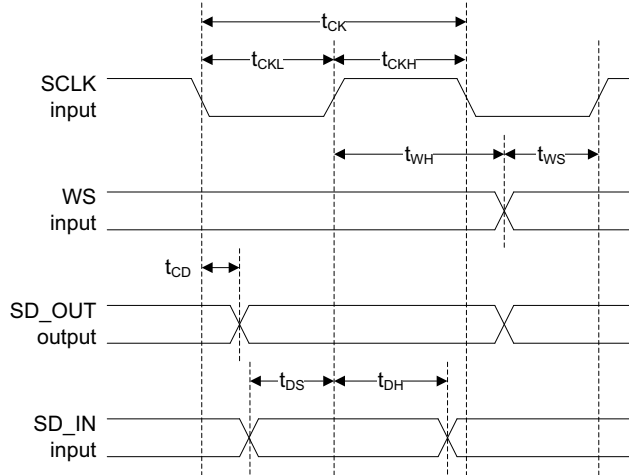
Figure 29: I2S slave mode timing diagram
