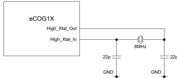
Figure 2: High reference oscillator external components
