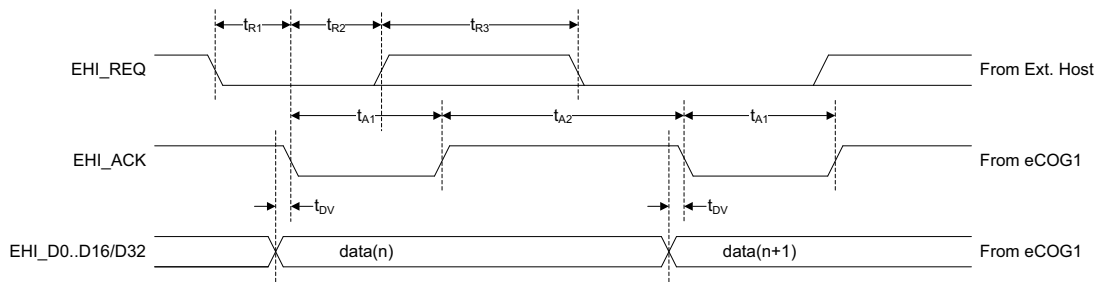
Figure 16: EHI DMA master read cycle timing diagram
