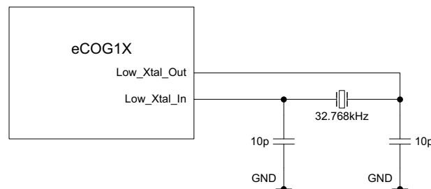
Figure 3: Low reference oscillator external components
