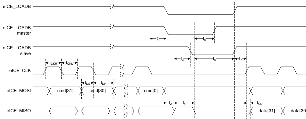
Figure 33: eICE read timing diagram
