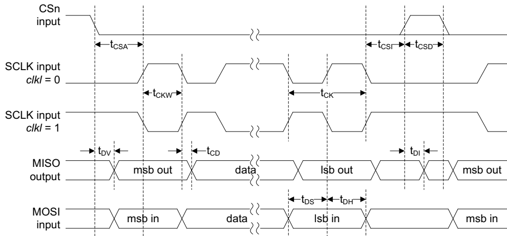
Figure 26: ESPI timing diagram, slave mode, cpha = 0
