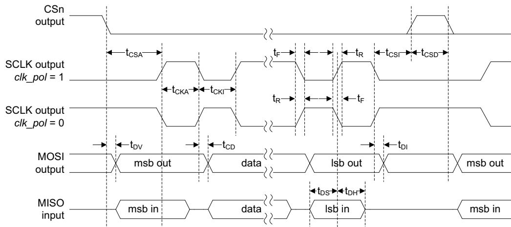
Figure 20: SPI timing diagram, master mode, clk\_pha = 0
