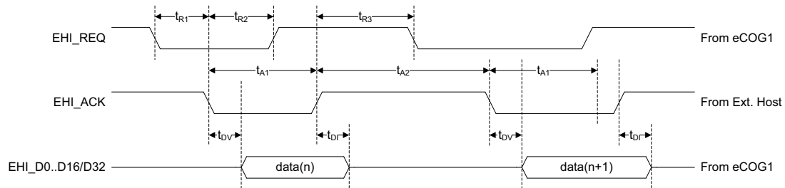
Figure 18: EHI DMA slave read cycle timing diagram
