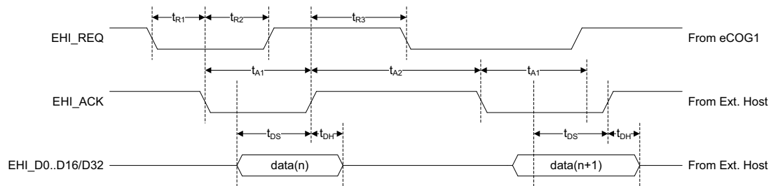
Figure 19: EHI DMA slave write cycle timing diagram
