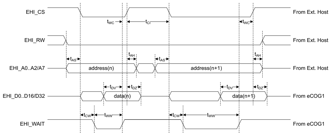
Figure 14: EHI MMP read cycle timing diagram
