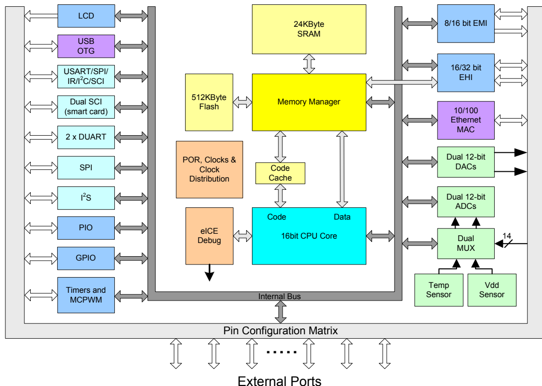
eCOG1X block diagram
