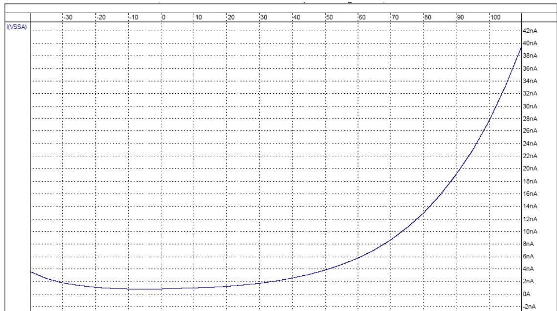
Figure 37: Voltage reference standby current with temperature (typical)
