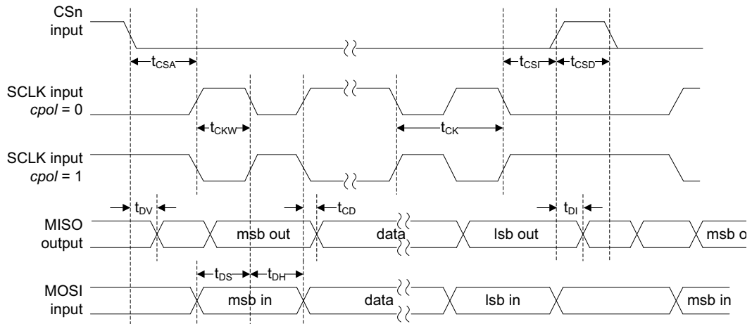
Figure 27: ESPI timing diagram, slave mode, cpha = 1
