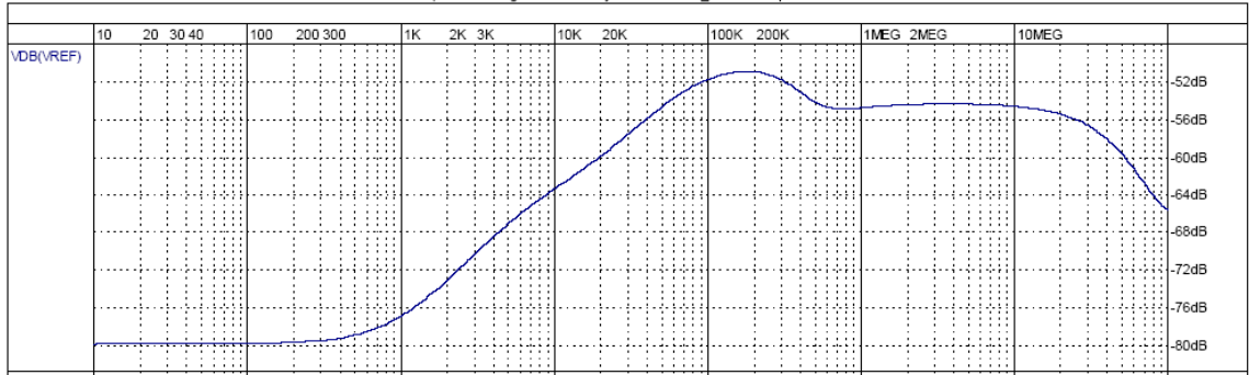
Figure 36: Vref supply noise rejection versus frequency (typical)
