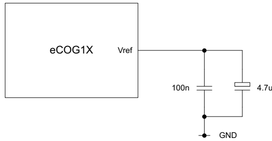
Figure 4: Vref decoupling
