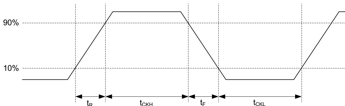
Figure 7: External clock source timing diagram
