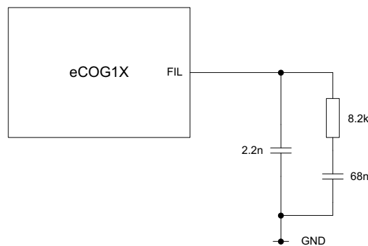
Figure 5: Low PLL filter external components
