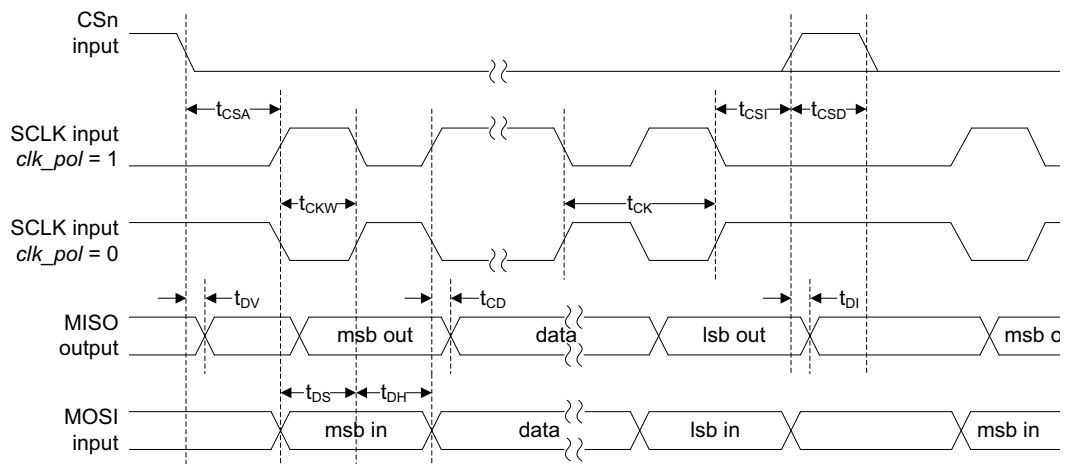
Figure 23: SPI timing diagram, slave mode, clk\_pha = 1
