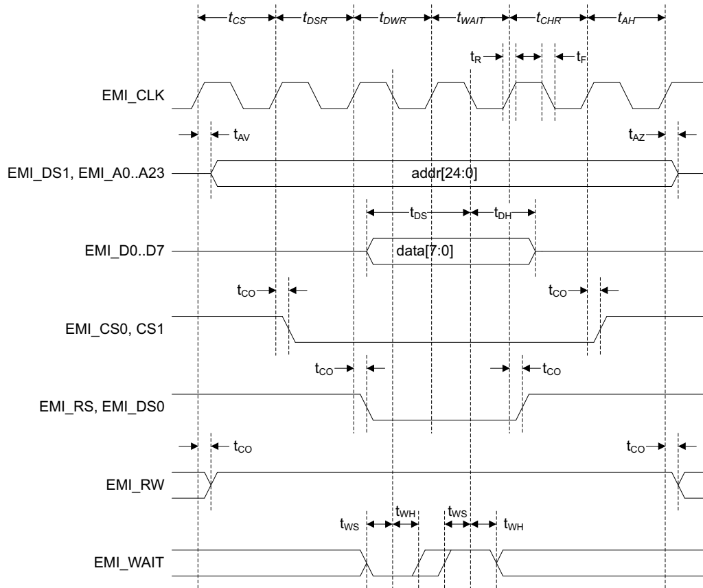
Figure 8: EMI bus mode 8-bit read cycle timing diagram
