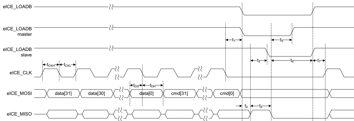
Figure 34: eICE write timing diagram
