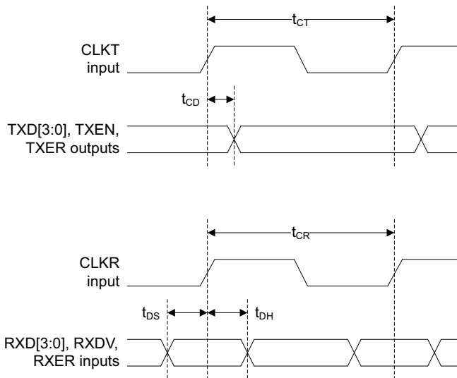
Figure 31: EMAC MII timing diagram
