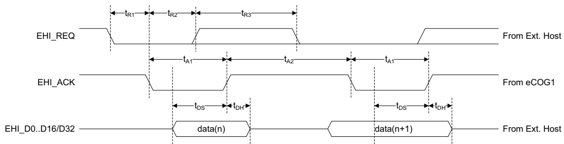
Figure 17: EHI DMA master write cycle timing diagram
