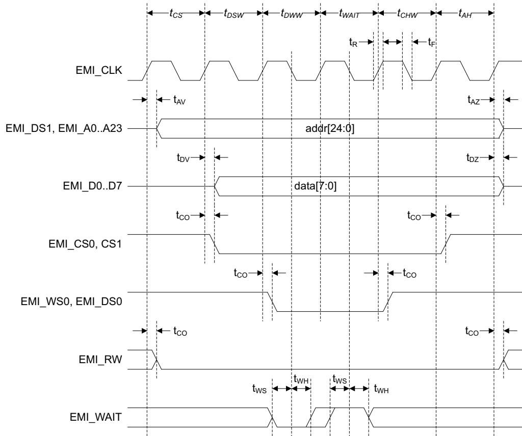
Figure 9: EMI bus mode 8-bit write cycle timing diagram
