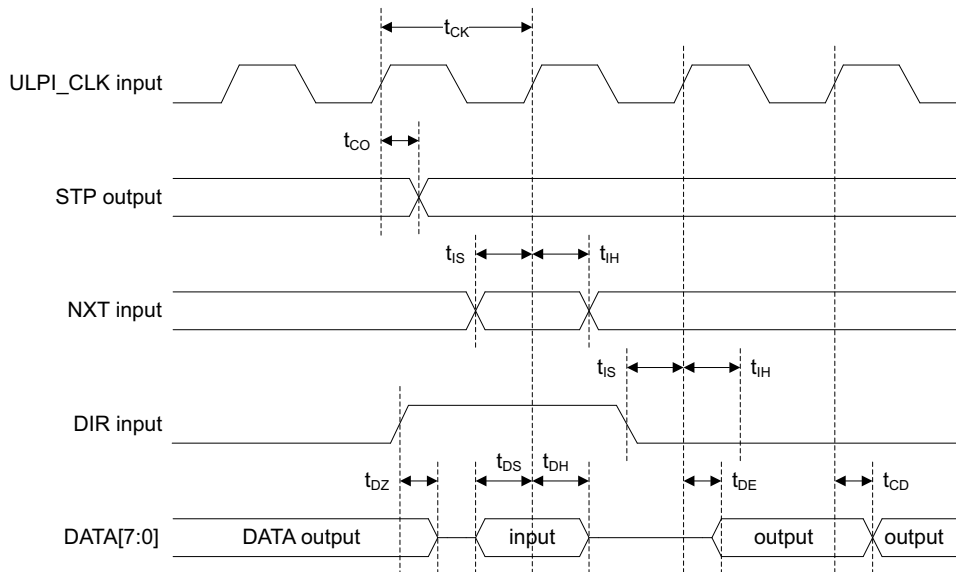
Figure 32: USB ULPI timing diagram
