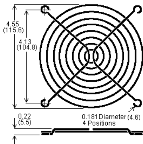
MC36424: Fan Kit (Fan, Wire Guard and Cord)
