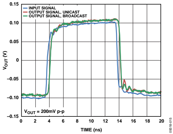
Figure 14. ADV3228 Small Signal Pulse Response
