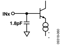
Figure 58. Analog Input
