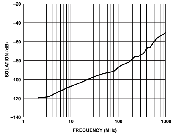
Figure 30. ADV3229 Off Isolation
