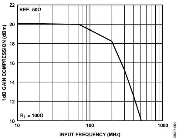
Figure 51. ADV3229 1 dB Gain Compression, 100 Ω Load
