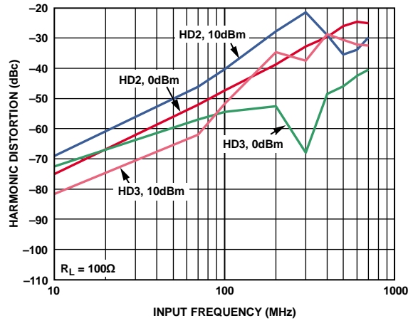
Figure 57. ADV3229 Harmonic Distortion, 100 Ω Load
