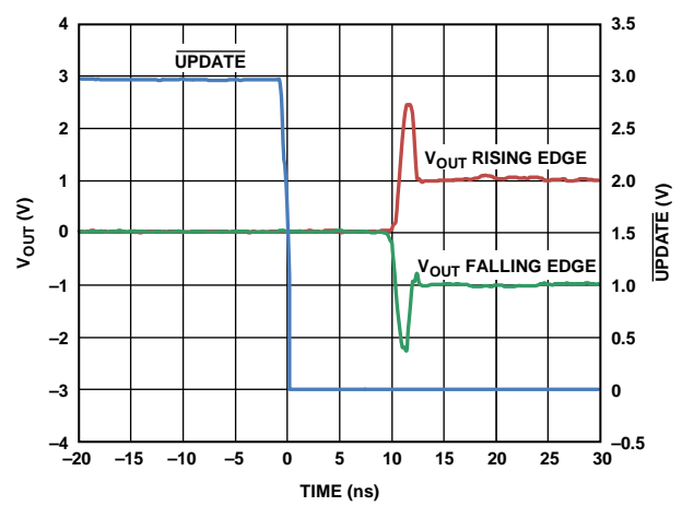
Figure 47. ADV3229 Enable Time
