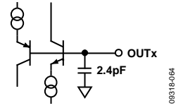
Figure 62. Analog Output Disabled
