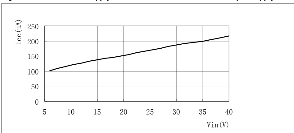
Figure 1.2 ZLED7020 Supply Quiescent Shutdown Current vs. Input Supply Voltage ( V_{IN} = 6 to 40 V)
