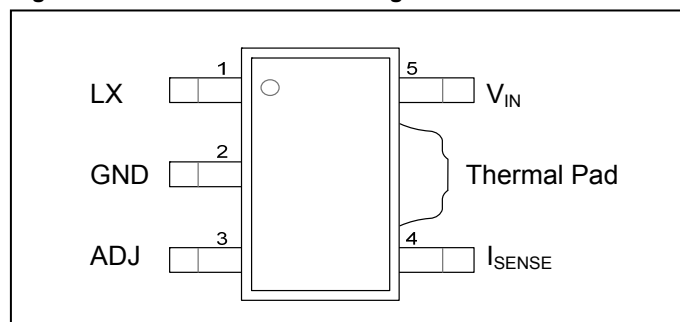
Figure 5.1 ZLED7020 Pin Configuration
