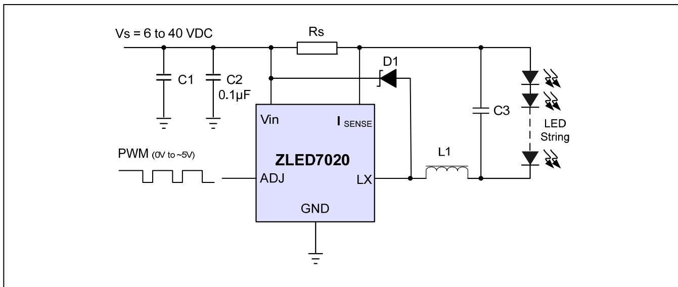
Figure 3.3 Basic ZLED7020 Application Circuit with Output Current Set by External Square Wave Voltage (PWM)
