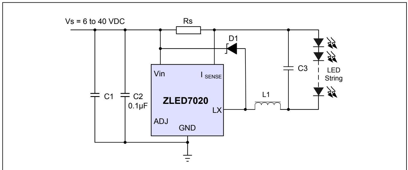
Figure 3.1 Basic ZLED7020 Application Circuit with Output Current Determined only by R_s
