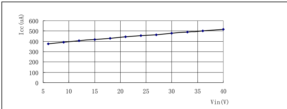
Figure 1.1 ZLED7020 Supply Operating Current vs. Input Supply Voltage ( V_{IN} = 6 to 40 V)
