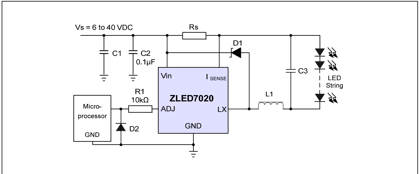
Figure 3.4 Basic ZLED7020 Application Circuit with Output Current Controlled by External Microcontroller Signal
