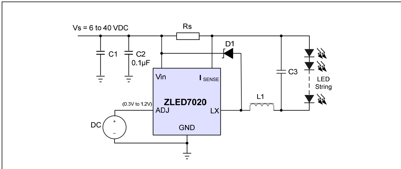
Figure 3.2 Basic ZLED7020 Application Circuit with Output Current Controlled by External DC Voltage
