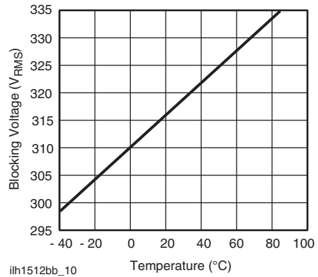
ih1512bb_10 Fig. 10 - Form B Typical Blocking Voltage vs. Temperature
