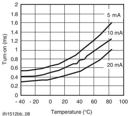
ih1512bb_08 Fig. 8 - Form A Typical Turn-On vs. Temperature
