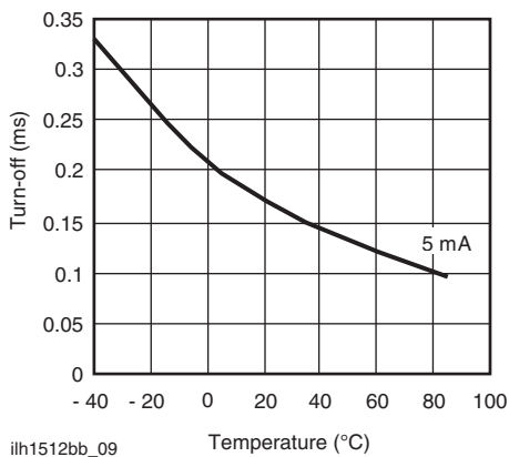
ih1512bb_09 Fig. 9 - Form A Typical Turn-Off vs. Temperature
