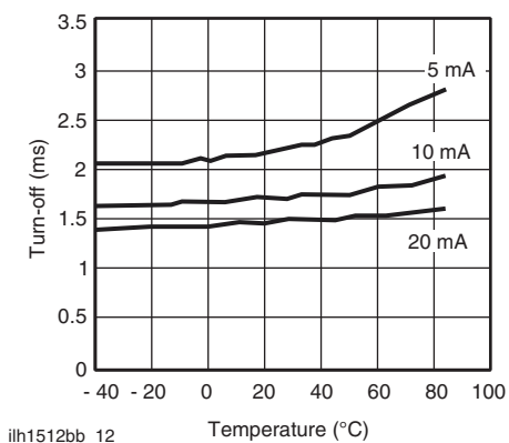
ih1512bb_12 Fig. 12 - Form B Typical Turn-Off vs. Temperature
