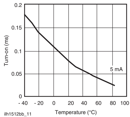
ih1512bb_11 Fig. 11 - Form B Typical Turn-On vs. Temperature
