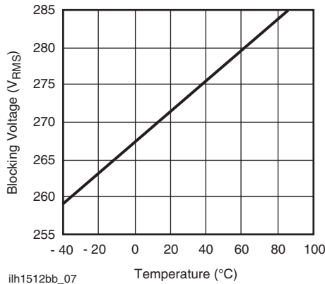
ih1512bb_07 Fig. 7 - Form A Typical Blocking Voltage vs. Temperature
