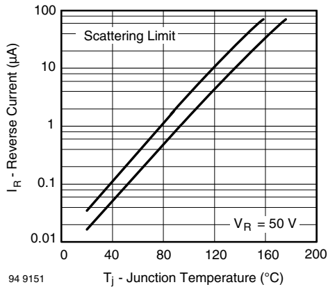
94 9151 T_j - Junction Temperature ( ^{\circ}\text{C} ) Figure 1. Reverse Current vs. Junction Temperature
