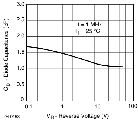
94 9153 V_R - Reverse Voltage (V) Figure 3. Diode Capacitance vs. Reverse Voltage
