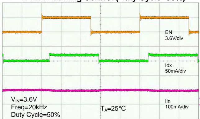
PWM Dimming Control (Duty Cycle=50%)
