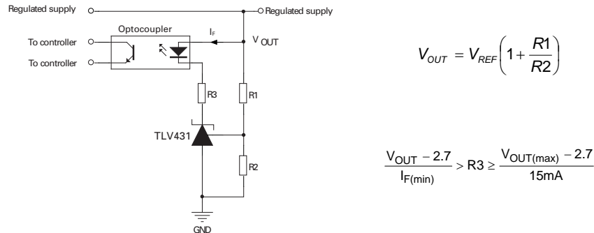
Figure 2. Using the TLV431 as the regulating element in an isolated PSU
