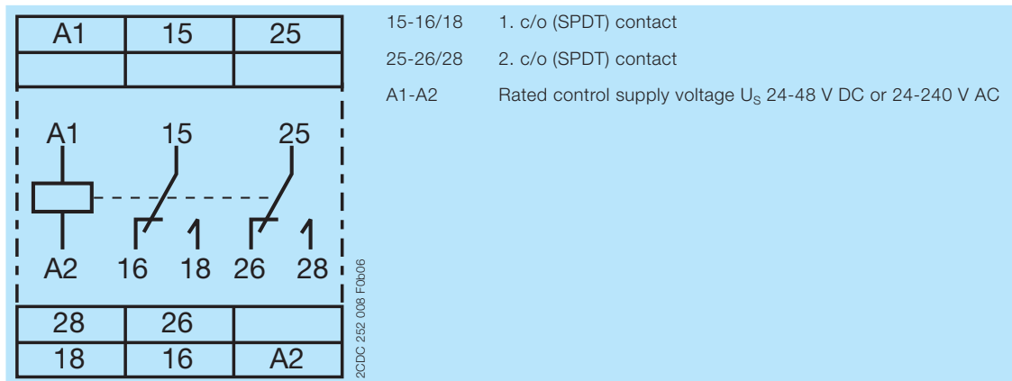
Connection diagram
