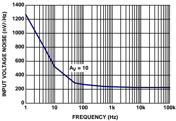
FIGURE 15. ISL28271 INPUT VOLTAGE NOISE SPECTRAL DENSITY
