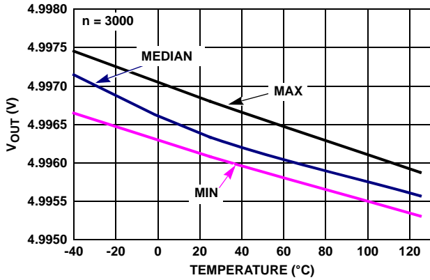
FIGURE 31. ISL28271 V_{OUT} HIGH vs TEMPERATURE, R_L = 100k , V_+ = \pm 2.5V
