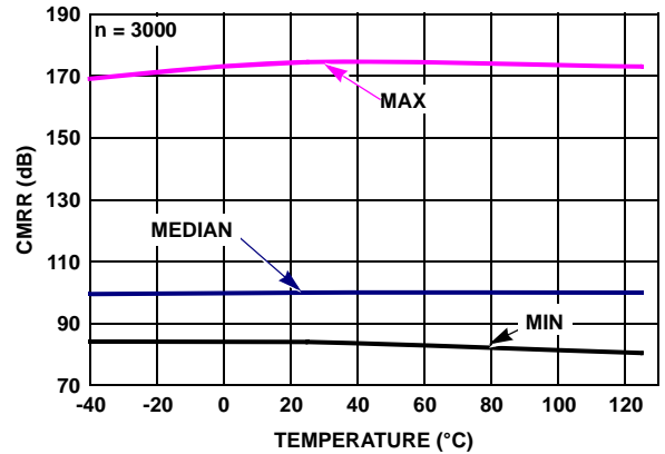
FIGURE 26. ISL28272 CMRR vs TEMPERATURE, V_{CM} = +2.5V TO -2.5V
