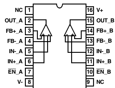
ISL28271, ISL28272 (16 LD QSOP) TOP VIEW
