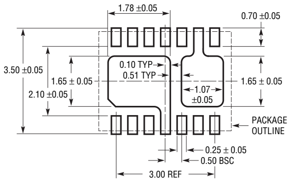
DE14MA Package 14-Lead Plastic DFN (4mm × 3mm) (Reference LTC DWG # 05-08-1731 Rev A)
