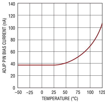
ADJP Pin Bias Current
