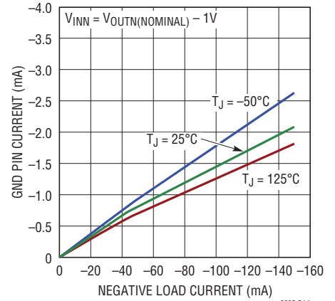
Negative Side GND Pin Current vs ILOAD
