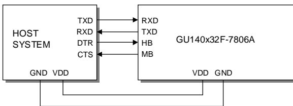
Host to Module Write
