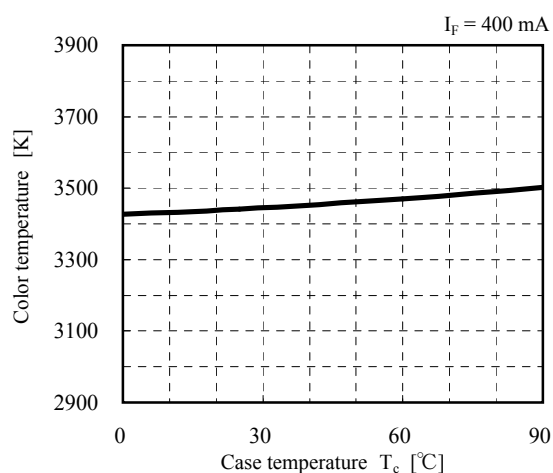
Case Temperature vs. Color Temperature
