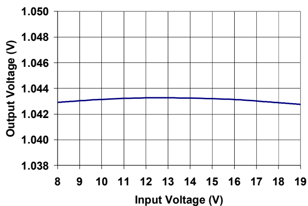
Figure 10: Line Regulation at I_{OUT} = 15A
