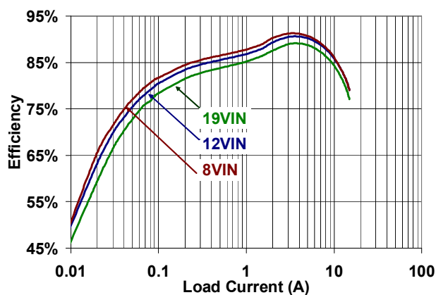
Figure 2: IR3477 Efficiency
