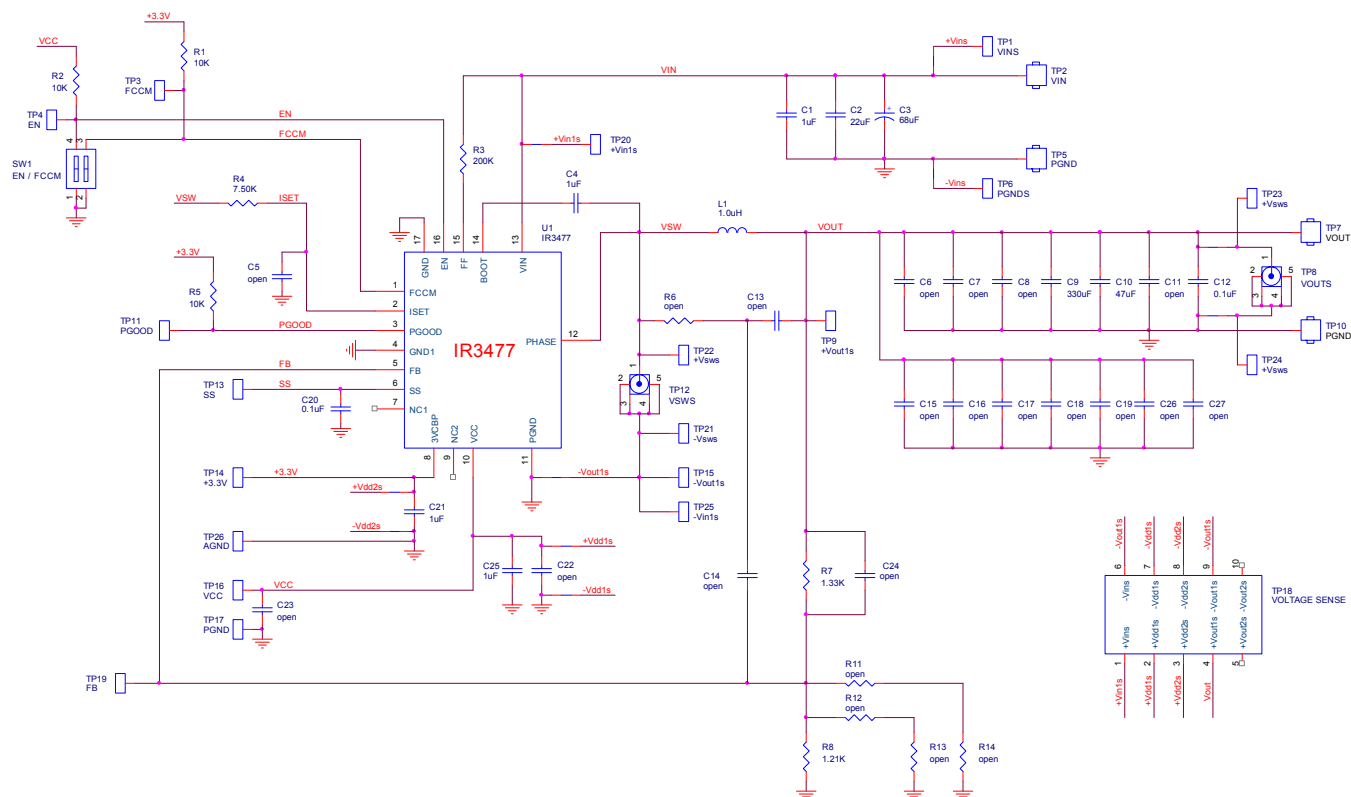
Figure 4: Demoboard Schematic for V_{OUT} = 1.05V , F_s = 300kHz
