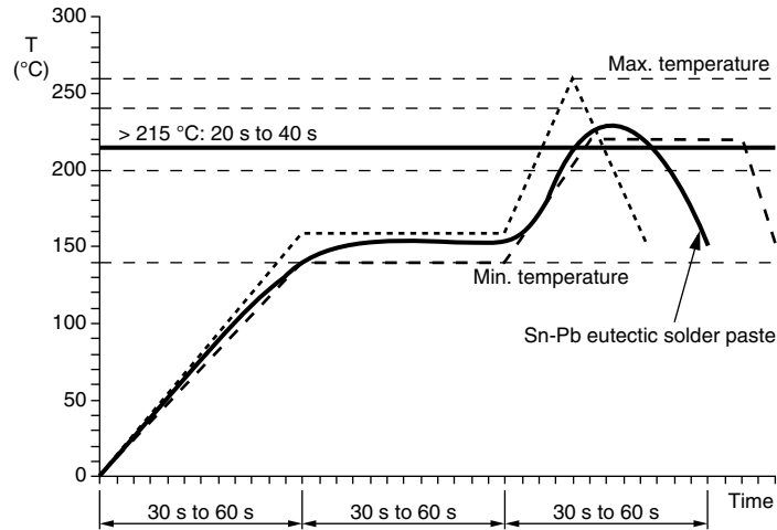
Fig. 6 - Soldering IR Reflow with SnPb Solder
