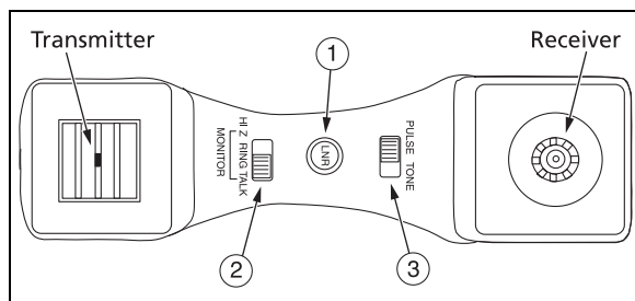
Figure 2. Handgrip Controls
