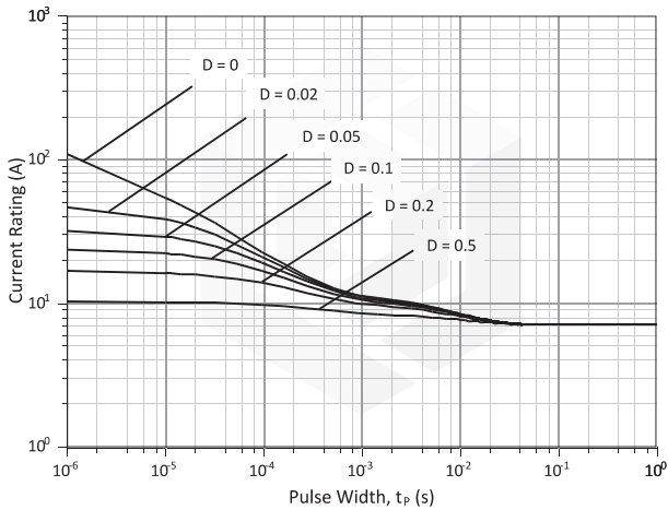
Figure 7: Typical Current versus Pulse Duration Curves at T_c = 200\text{ }^\circ\text{C}
