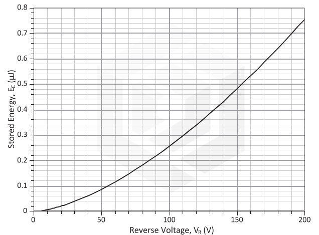
Figure 6: Typical Switching Energy versus Reverse Voltage Characteristics
