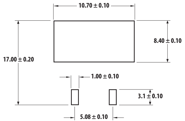
Figure 15. Recommended soldering land pattern
