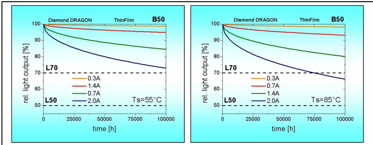
Figure 8d: Degradation characteristics (6) of the Diamond DRAGON with ThinFilm technology for T_s = 55^\circ\text{C} and T_s = 85^\circ\text{C} (grouping current I_F = 1.4\text{ A} )
