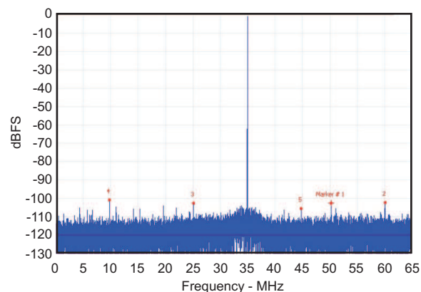
Figure 42. FFT Plot of THS770012 + 30MHz BPF + ADS5493 with 95MHz Single-Tone Input Sampling at 130MSPS
