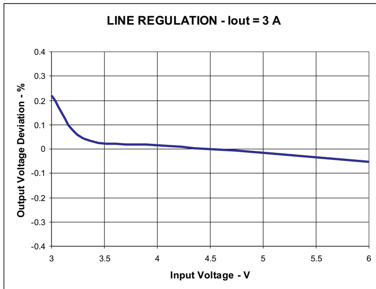
Figure 4. TPS54618EVM-606 Line Regulation
