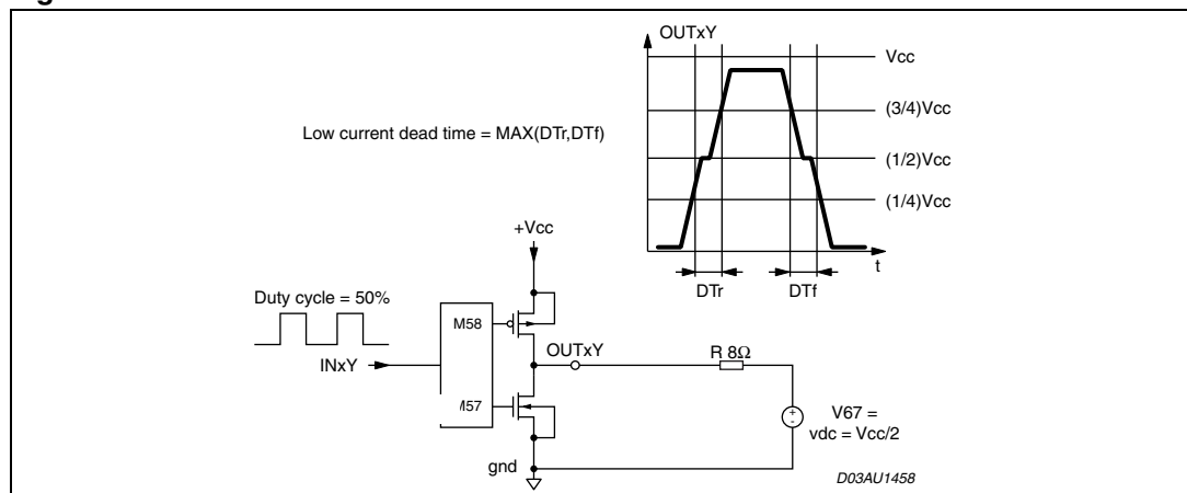
Figure 4. Resistive load
