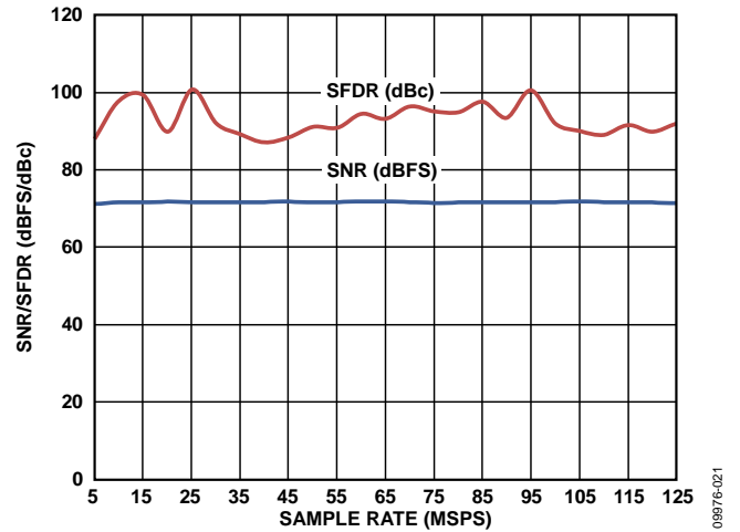
Figure 19. SNR/SFDR vs. Sample Rate with AIN = 70 MHz
