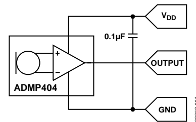
Figure 1. Evaluation Board Schematic
