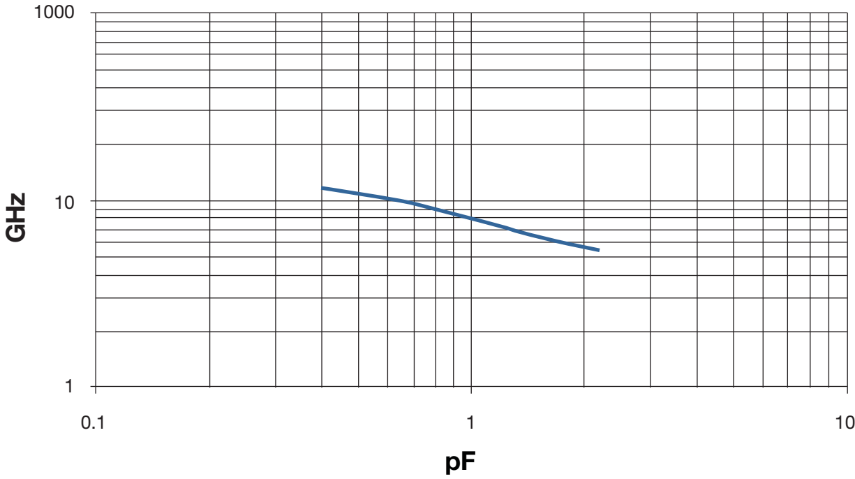
Typical Self Resonant Frequency vs Capacitance OPC 0603
