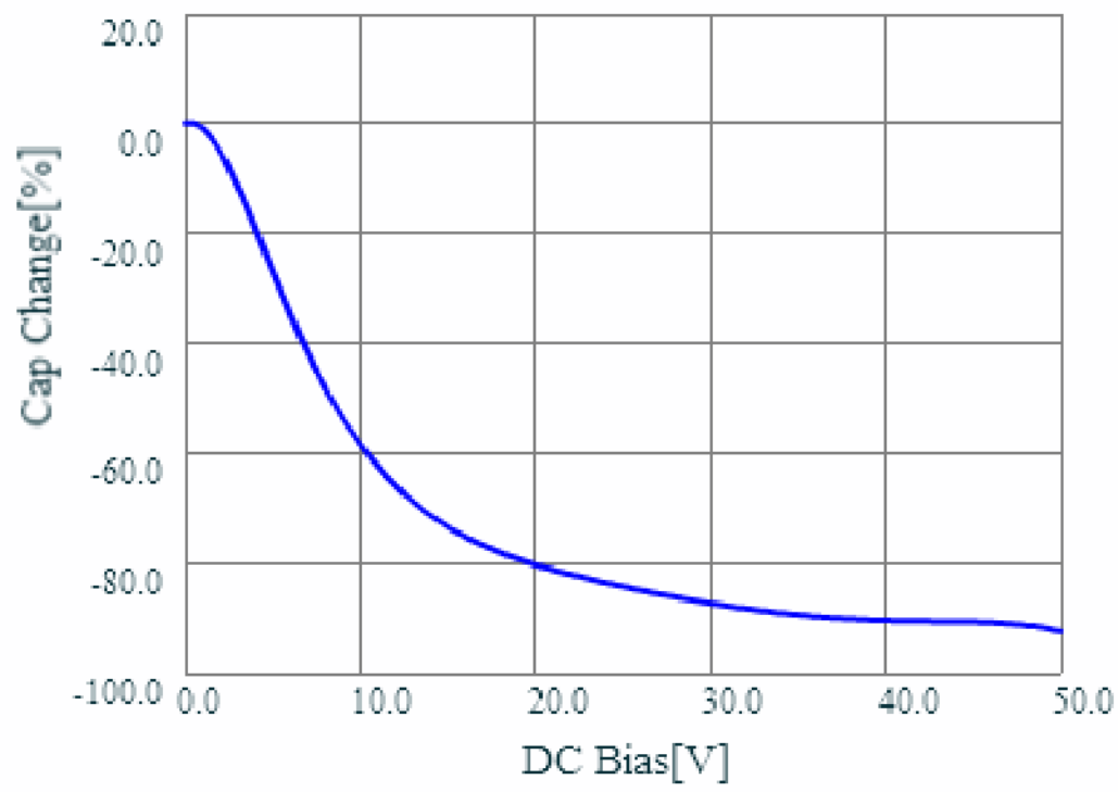
GRM31CR61H106KA12 C-DC bias.Cap Change
