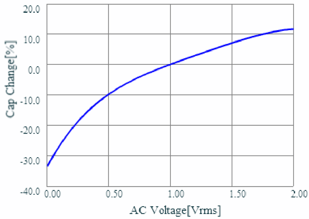
GRM31CR61H106KA12 C-AC Voltage.Cap Change
