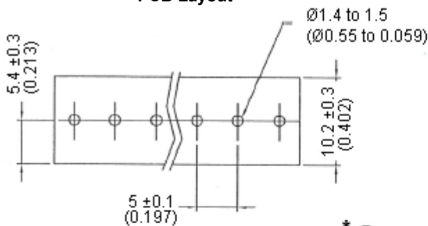
PCB Layout
