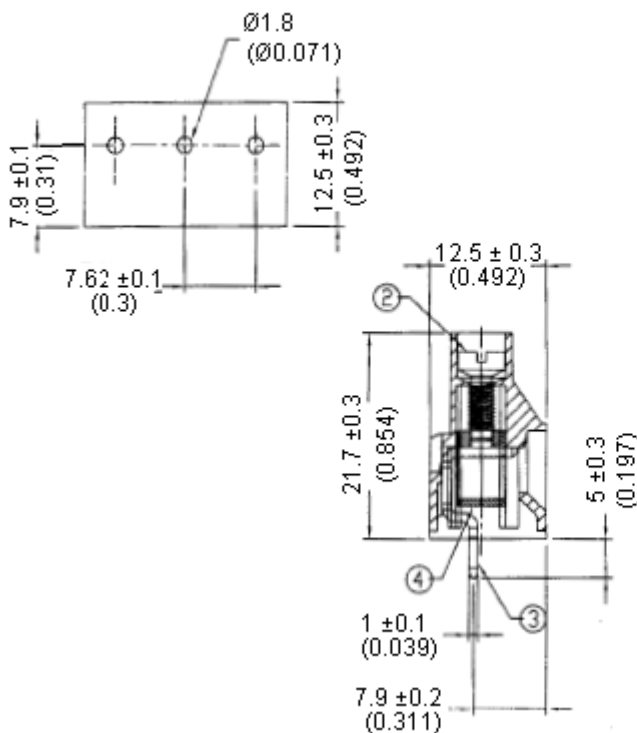
PCB Layout
