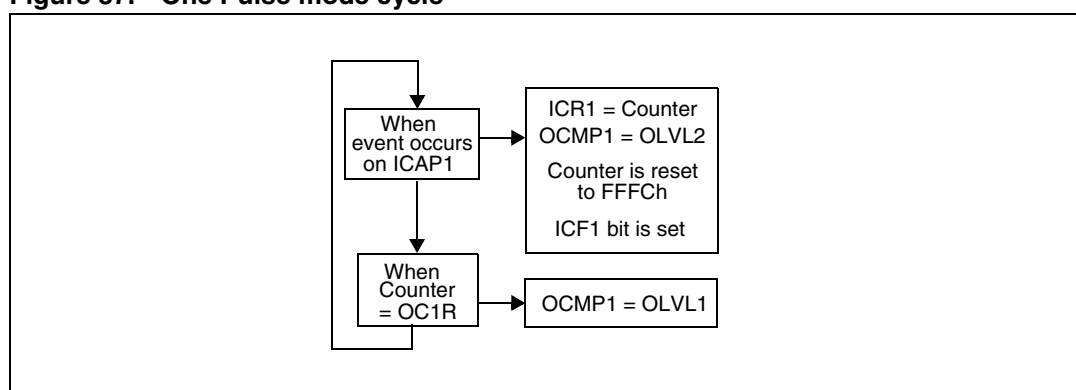
Figure 37. One Pulse mode cycle
