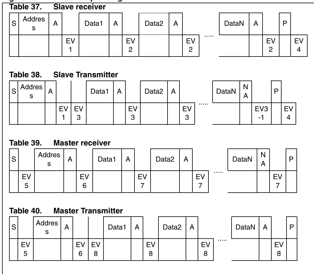
Figure 48. Transfer sequencing
