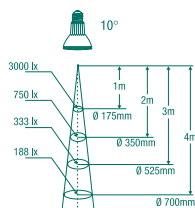
Hi-Spot 80 50W/10°
