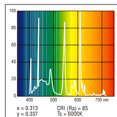
Daylight Deluxe 860
