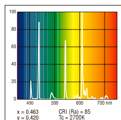
Homelight Deluxe 827
