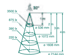
Hi-Spot 120 100W/30°
