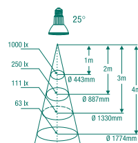
Hi-Spot 80 50W/25°
