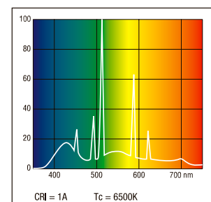
Reptistar
