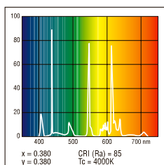
Coolwhite Deluxe 840
