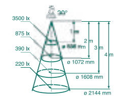
Hi-Spot 95 100W/30°
