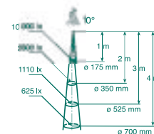
Hi-Spot 120 100W/10°
