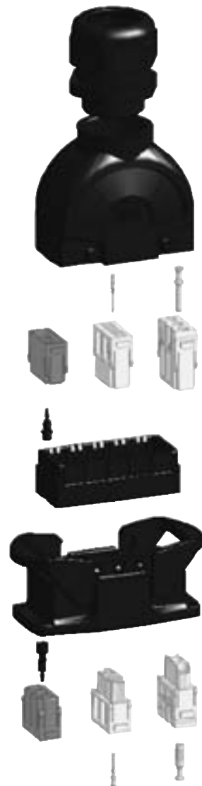
Assembly details
