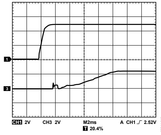
Figure 23. Power-On Reset to Midscale
