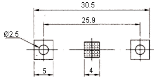
PCB Mounting Layout
