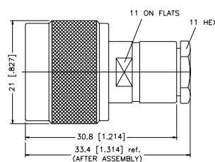
Assembly Instruction M - page 235
