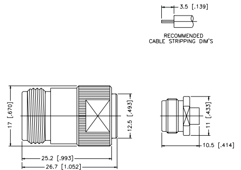
Assembly Instruction G - page 229
