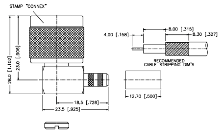
Assembly Instruction I - page 231
