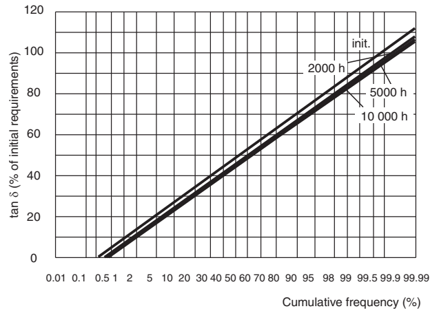
Fig. 11 - tan δ change of capacitance as a function of cumulative frequency after endurance test
