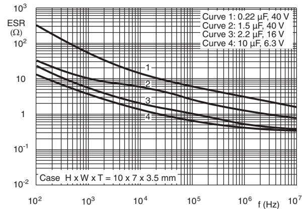
Fig. 13 - Typical ESR at 25 °C as a function of frequency
