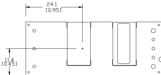
Figure 22. Pick and Place Location.
