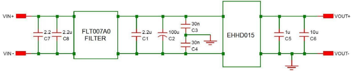
Figure 27. EMC Considerations
