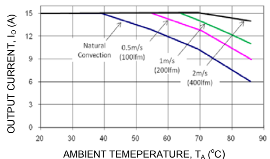
Figure 18. Output Current Derating for the Open Frame Module; Airflow in the Transverse Direction from V_{out(-)} to V_{out(+)} ; V_{IN} = 24V , V_O = 5.0V .
