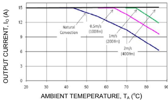
Figure 19. Output Current Derating for the Module with Heatplate; Airflow in the Transverse Direction from V_{out(-)} to V_{out(+)} ; V_{IN}=24V , V_O=5.0V .
