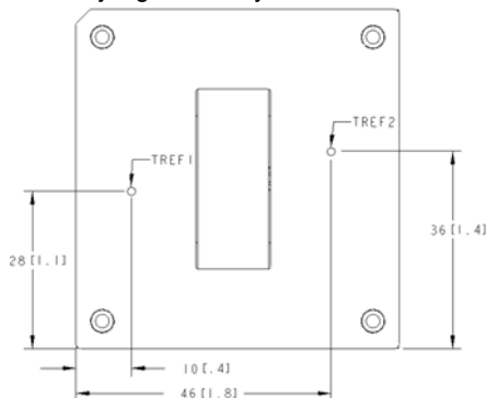
Figure 17. Case ( T_{REF} ) Temperature Measurement Location (top view).
