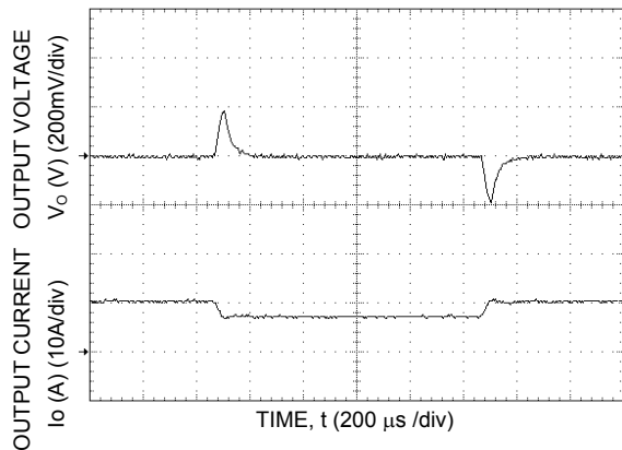
Figure 3. Transient Response to Dynamic Load Change, 0.1A/µs, from 75% to 50% to 75% of full load.
