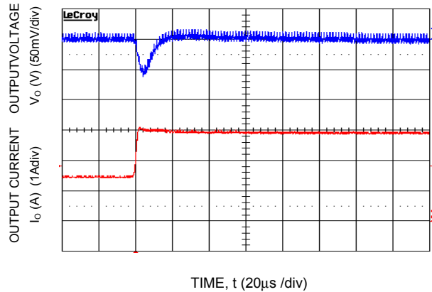
Figure 28. Transient Response to Dynamic Load Change from 50% to 100% at 12V in , C out -2x47μF, CT tune -2200pF & RT tune -261
