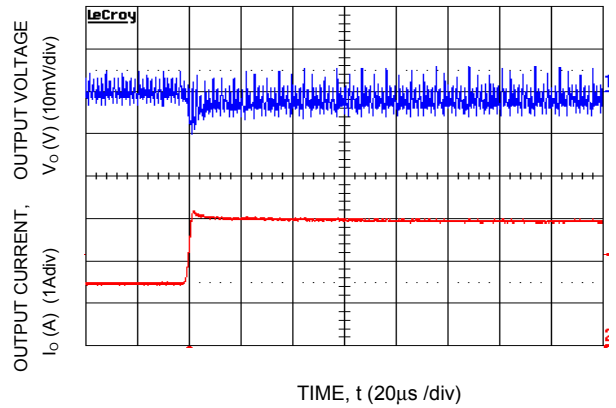
Figure 4. Transient Response to Dynamic Load Change from 50% to 100% at 12Vin, C_{out}=1x47\mu\text{F}+2x330\mu\text{F} , C_{Tune}=27\text{nF} , R_{Tune}=178
