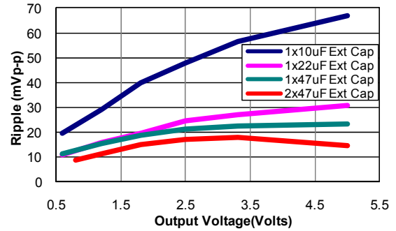
Figure 38. Output ripple voltage for various output voltages with external TBD ceramic capacitors at the output (3A load). Input voltage is 12V.
