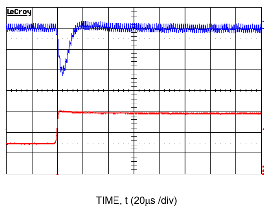
Figure 34. Transient Response to Dynamic Load Change from 50% to 100% at 12Vin, C_{out}=1x47\mu F , C_{Tune}=820pF & R_{Tune}=261
