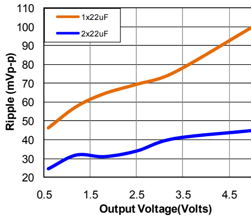
Figure 37. Input ripple voltage for various output voltages with TBD \mu\text{F} or TBD \mu\text{F} ceramic capacitors at the input (3A load). Input voltage is 12V.
