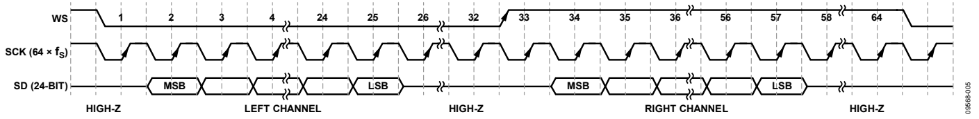
Figure 10. Stereo Output I 2 S Format
