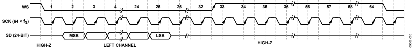
Figure 11. Mono Output I 2 S Format Left Channel (L/R = 0)
