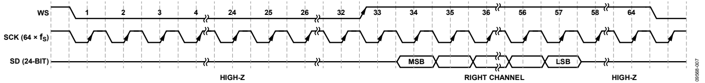
Figure 12. Mono Output I 2 S Format Right Channel (L/R = 1)
