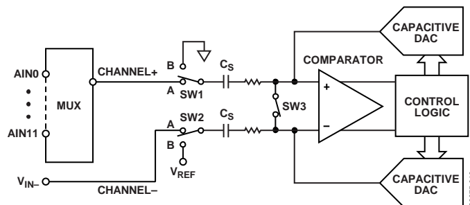
Figure 25. ADC in Pseudo Differential Mode
