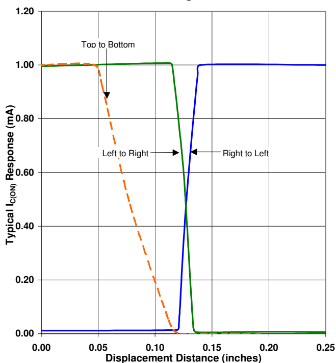
OPB820S10 - Flag Next to Sensor
