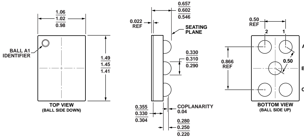
Figure 36. 5-Ball Wafer Level Chip Scale Package [WLCSP] (CB-5-3) Dimensions shown in millimeters
