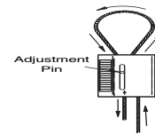
Step 5 To adjust, remove tension and pull wire rope slightly to disengage teeth, slide adjustment pin in direction shown by arrow to release wire rope
