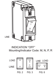
MARKING DETAIL "C" (SEE TABLE)
