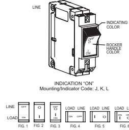
MARKING DETAIL "B" (SEE TABLE)
