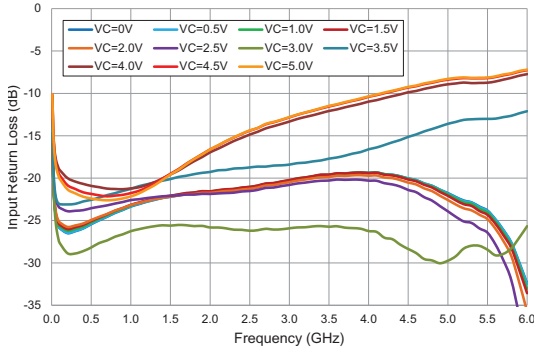
Input Return Loss versus Frequency V_{DD}=5V , Temp=+25°C
