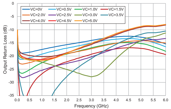
Output Return Loss versus Frequency V_{DD}=5V , Temp=+25°C
