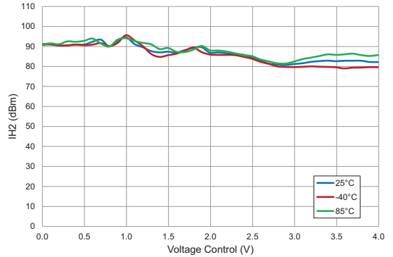
2nd Harmonic IH2 versus Voltage Control RF 2GHz, V_{DD}=5V , P_{in}=+20dBm
