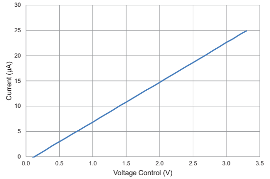
VC Pin Current versus Voltage Control Negative Slope, MODE=Low, V_{DD}=5V
