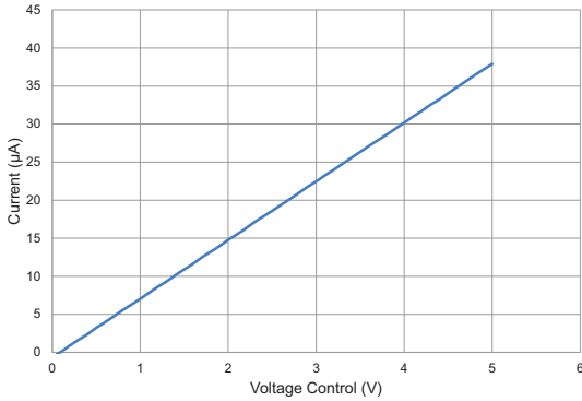
VC Pin Current versus Voltage Control Positive Slope, MODE=High, V_{DD}=5V
