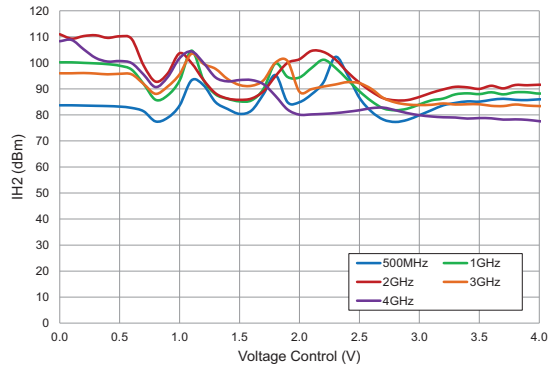
2nd Harmonic IH2 versus Voltage Control V_{DD}=5V , P_{in}=+20dBm , Temp= +25^{\circ}C
