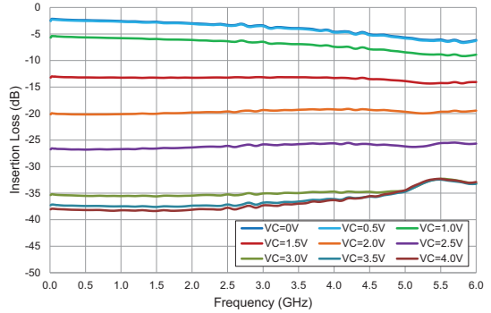
Insertion Loss versus Frequency V_{DD}=5V , Temp=+25°C
